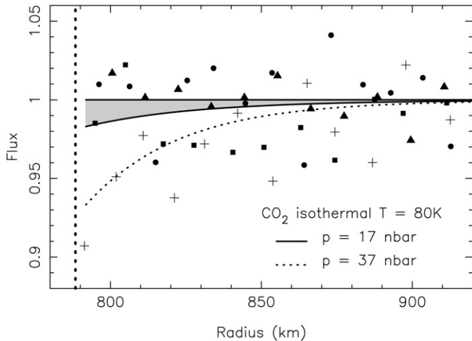
Fig. 15. Same as Fig. 5, but at different scales, to illustrate the effect of a faint atmosphere on the light curves. Symbols are the same as in Fig. 5, namely Salinas-1 0.25 m (squares), Salinas-2 0.20 m (bullets), Arikok 0.20 m (triangles) and Portimão-1 0.25 m (crosses). For each of the four lightcurves, the before-ingress and after-ingress data points have been folded over and binned over \sim 20 km vertical bins, in order to take into account the relative velocity of the star perpendicularly to each limb, so that the radial sampling \Delta r is constant at each station on the plot. In this way the actual contribution of stations to vertical sampling can be assessed, although the fit to model was performed on actual data points. The point on left (Portimão) corresponds to the stellar drop behind Titania's limb at r < 792 km (those data points were not included in the fit). The dotted vertical line corresponds to our estimate of Titania's radius best value of 788.4 km. The smooth solid line is the 1- \sigma upper limit for the fit of actual data points to a CO 2 isothermal ( T = 80 K) model atmosphere, with a surface pressure of 17 nbar. The dotted line is the 3- \sigma upper limit ( p = 27 nbar). The shaded area shows the difference between this model and an airless model. See Table 5 and text for details.
